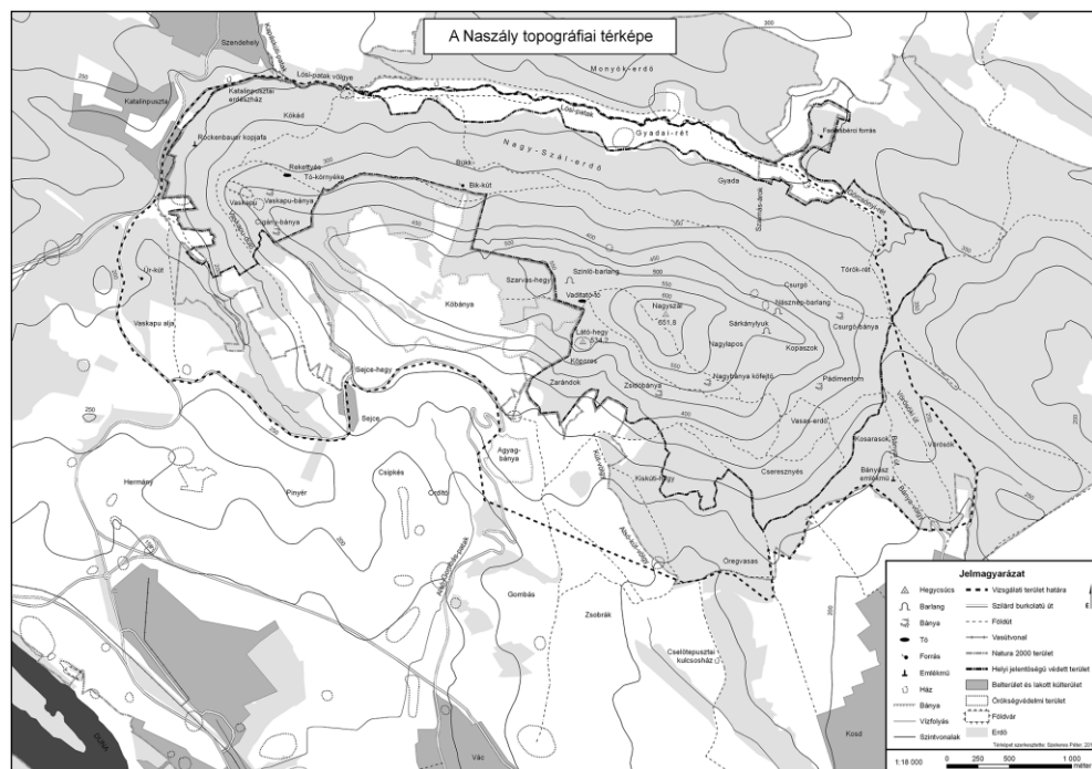
Figure 1. The research area of Naszály, its border with dashed line (PINTÉR & TÍMÁR 2010; map by P. SZEKERES)
